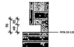
5 DET. FITA LED BANCADA 1:5
